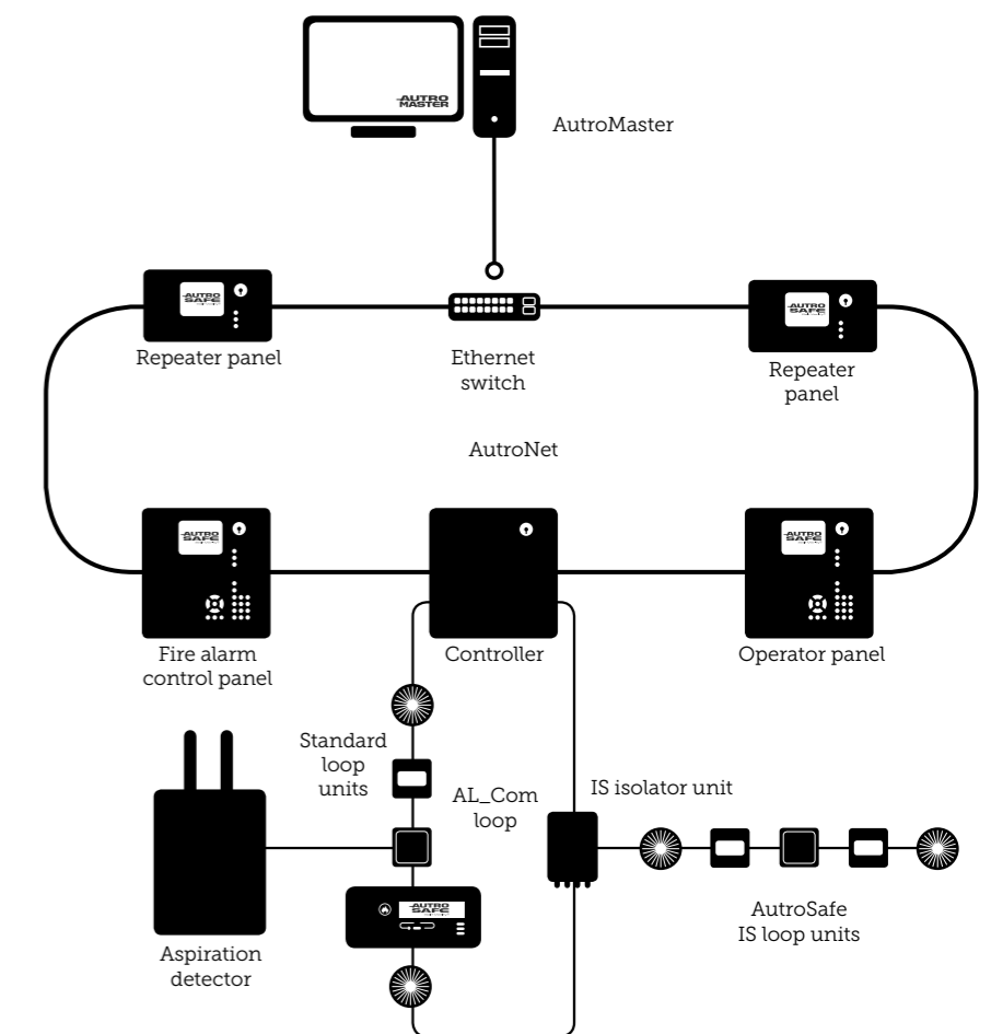
Star topology
